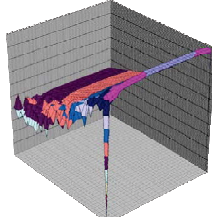
Figure 36. BUCK MINI Efficiency C_O = 100\mu\text{F} , L = 33\mu\text{F} Automatic Mode
